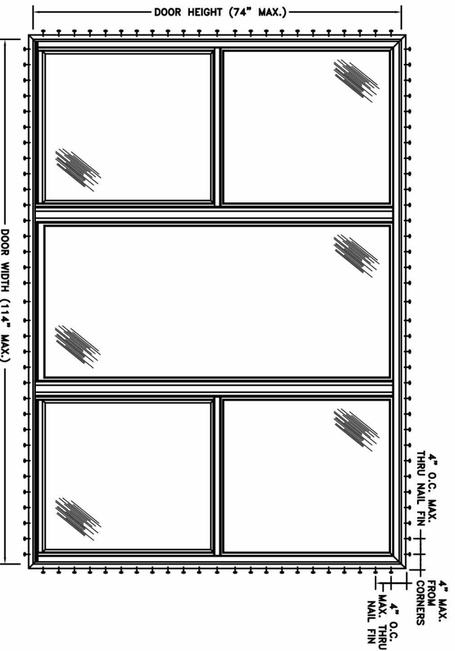
TYPICAL ELEVATION WITH FASTENER SPACING
